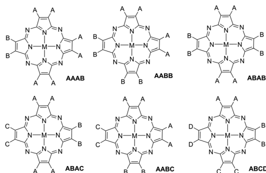
Fig. 1 General structures for non-uniformly substituted tetraazaporphyrins.
